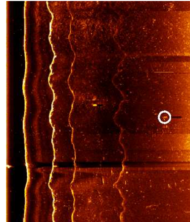
Fig. 1. A sample object (circled) in a partial sidescan sonar image with its shadow to the right.
